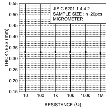
Fig.4 Dimensions (thickness)
