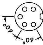
DIN 5 pin 240° Fully Screened Line Socket. 2001
