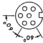
DIN 6 pin Fully Screened Line Socket. 2006
